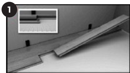
STEP 1: Lock short edge of plank by inserting tongue into groove
